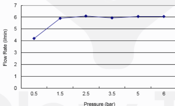
Flow Rate Chart of Armitage Shanks A4672AA
